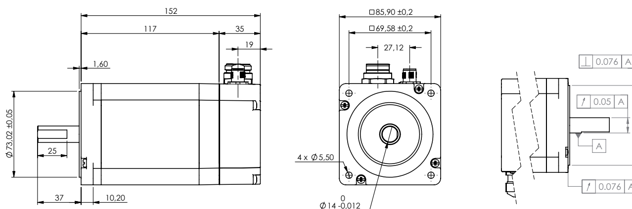
IP65 motor housing, except output flange
